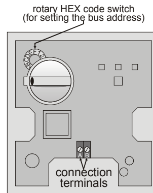
Fig. 2. SDW 10 (with front panel removed)
