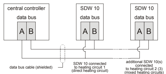
Fig. 3. Connecting to a central controller
